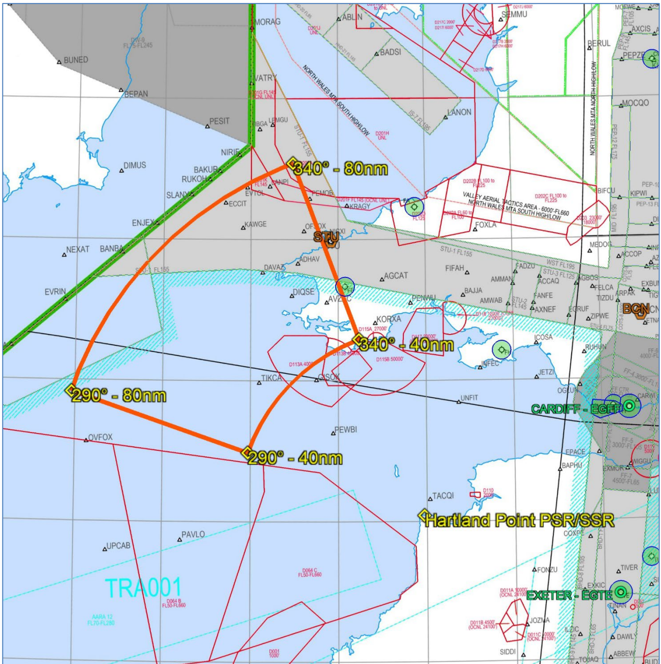
Chart 9 – SSR 5,000ft (80nm – 40nm)
