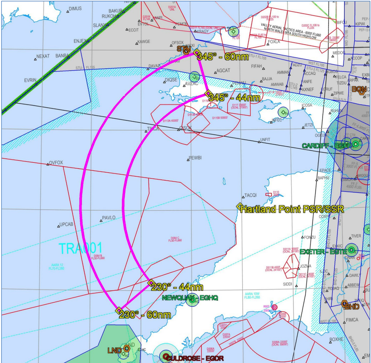
Chart 7 – PSR 22,000ft (60nm – 44nm)
