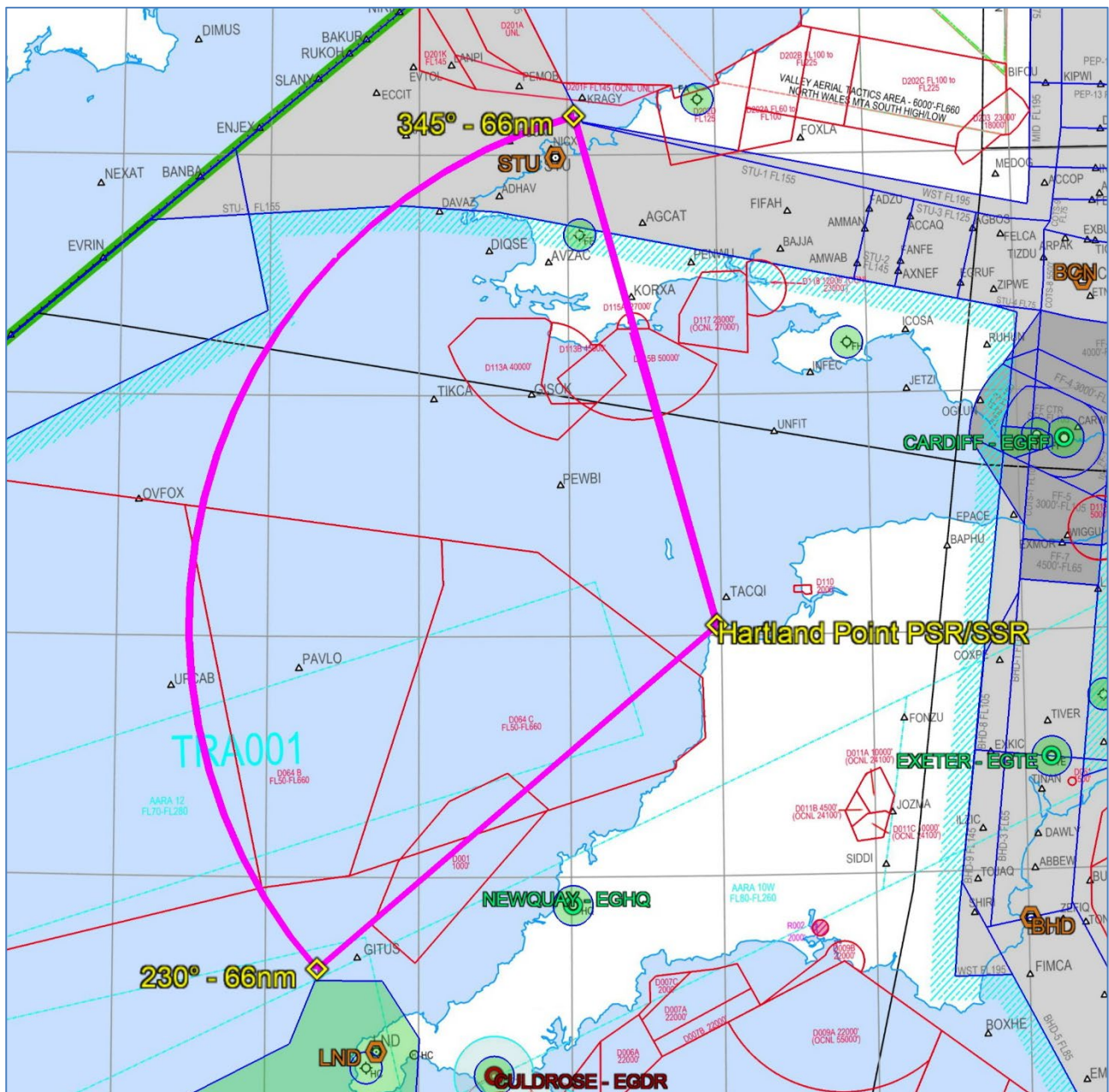
Chart 6 – PSR 22,000ft (66nm – OH)
