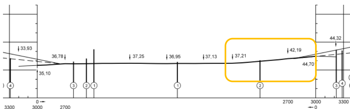
Figure 4: Typical example of 'complex' mean LSAA slope greater than 0.8 % but lower than 1 % (EDDL 23L dated 2009)
