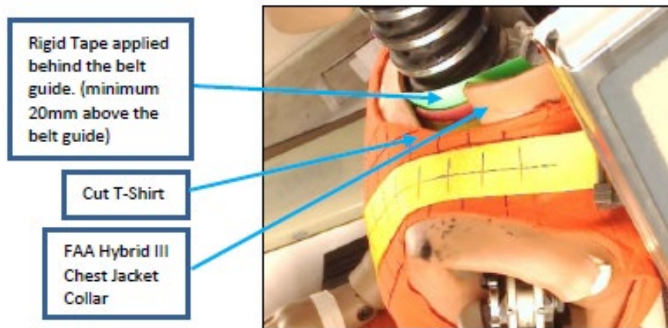
Figure 5 - Identification of Contact with Belt Guide on FAA HIII ATD
