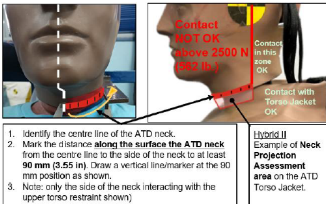
Figure 9 - Hybrid II ATD Marking to facilitate identification of contact
