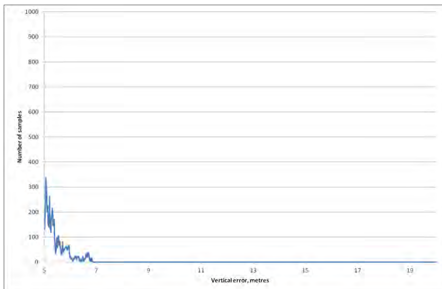
Figure 3-4: Vertical Error Distribution above 5m for Monitoring Period
