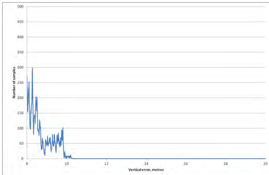
Figure 3-4: Vertical Error Distribution above 8m for Monitoring Period
