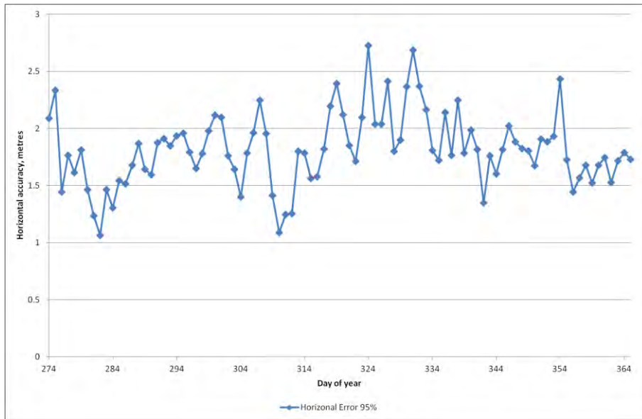
Figure 3-5: Horizontal Position Accuracy (95%) for Monitoring Period
