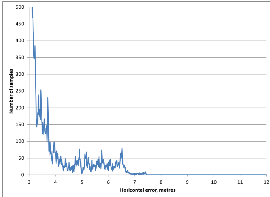
Figure 3-3: Horizontal Error Distribution after 3m for Monitoring Period
