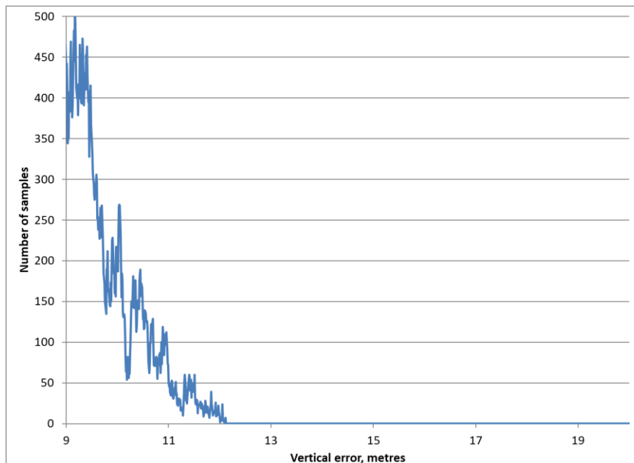
Figure 3-4: Vertical Error Distribution above 9m for Monitoring Period
