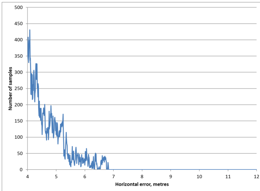
Figure 3-3: Horizontal Error Distribution after 4m for Monitoring Period
