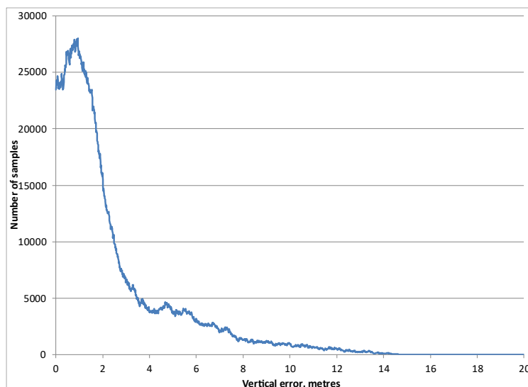
Figure 3-2: Vertical Error Distribution for Monitoring Period
