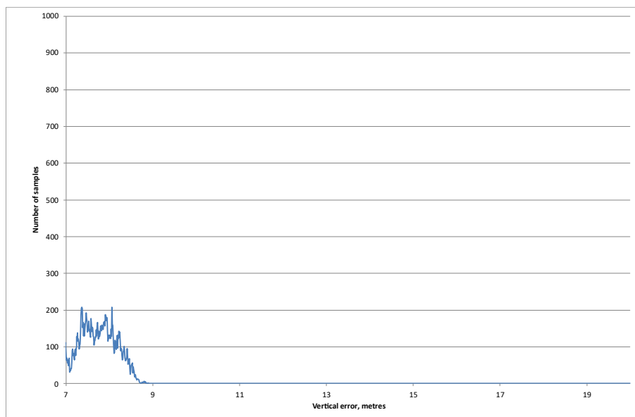
Figure 3-4: Vertical Error Distribution above 7m for Monitoring Period
