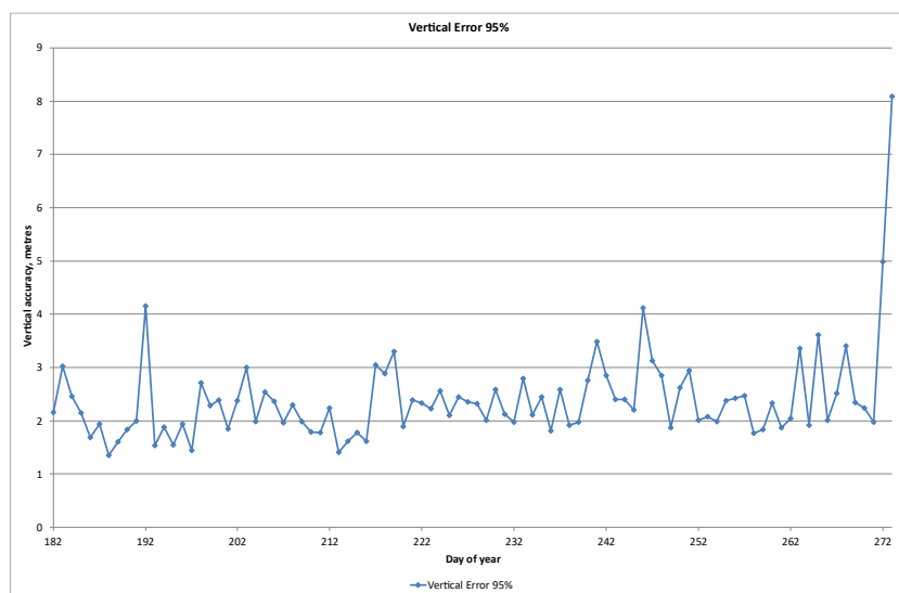
Figure 3-6: Vertical Position Accuracy (95%) for Monitoring Period
