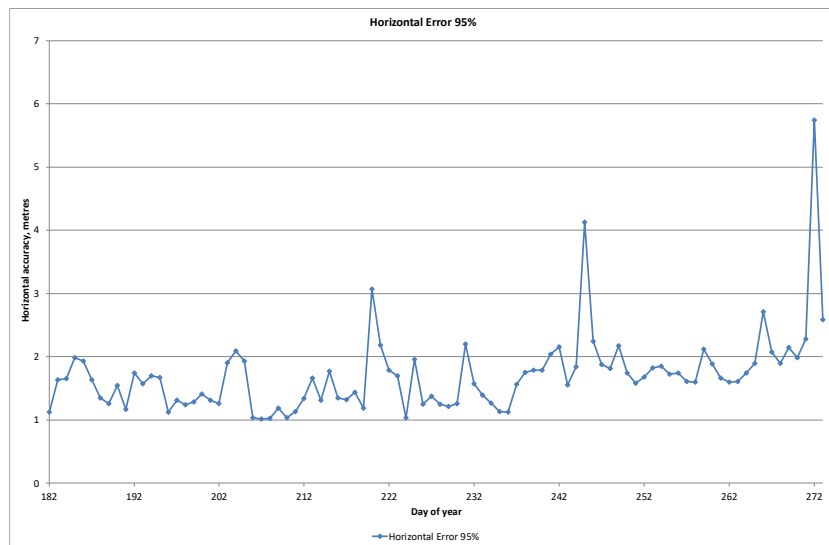
Figure 3-5: Horizontal Position Accuracy (95%) for Monitoring Period
