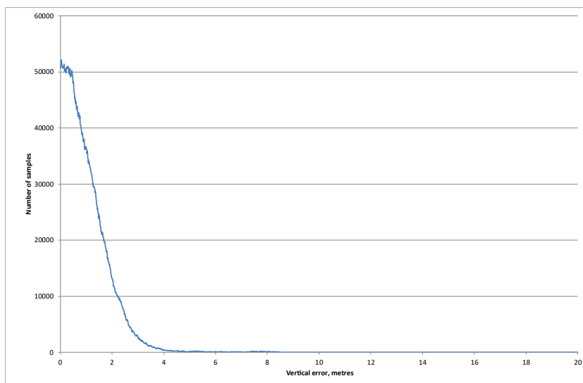
Figure 3-2: Vertical Error Distribution for Monitoring Period
