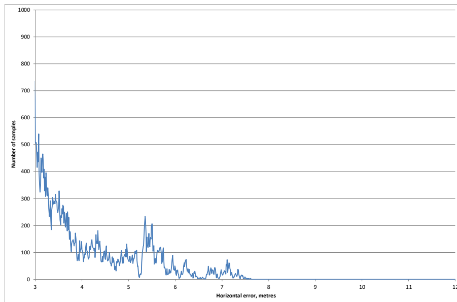
Figure 3-3: Horizontal Error Distribution after 3m for Monitoring Period
