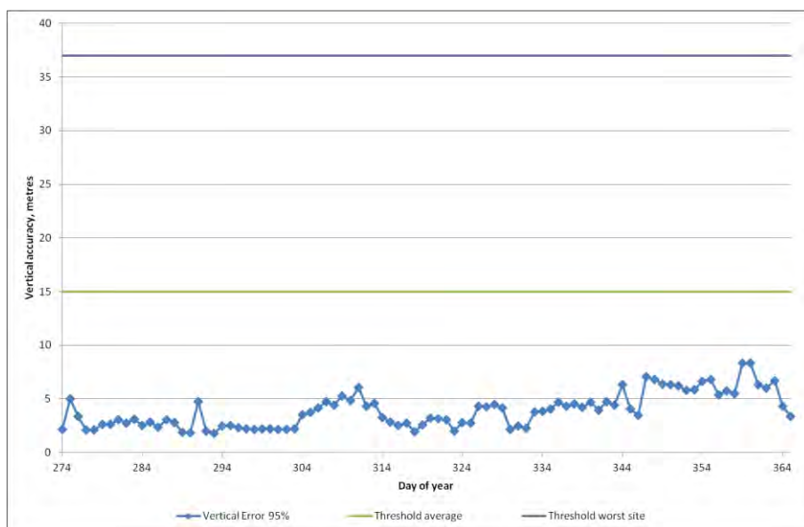
Figure 3-8: Daily Vertical Position Accuracy (95%) for Reporting Period
