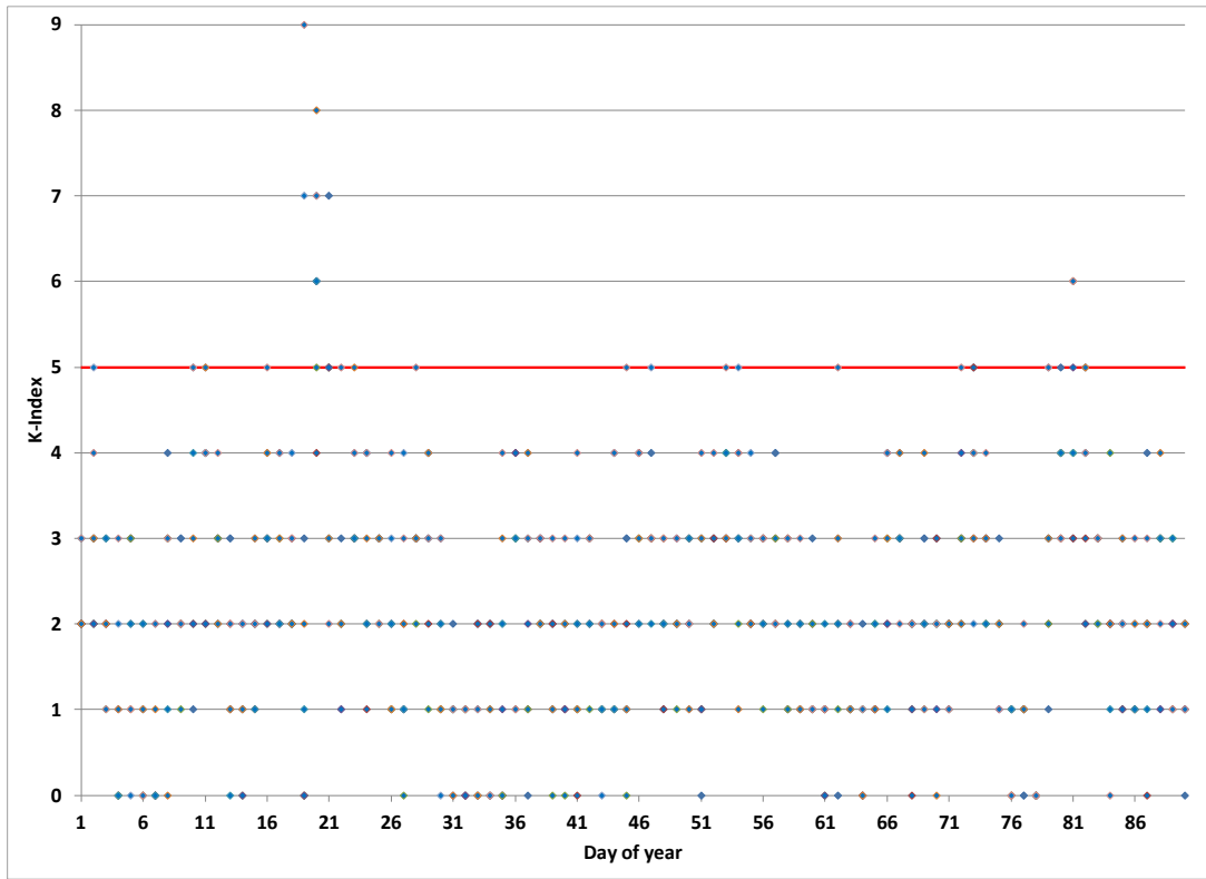
Figure 5-2: K-Index Values at Eskdalemuir during Reporting Period
