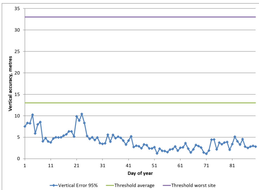
Figure 3-8: Daily Vertical Position Accuracy (95%) for Reporting Period L1 only
