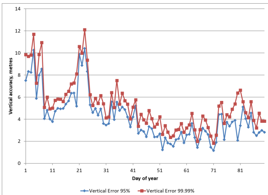
Figure 3-10: Daily Vertical Position Accuracy (99.99%) for Reporting Period L1 only
