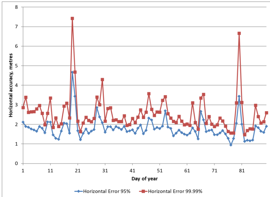
Figure 3-9: Daily Horizontal Position Accuracy (99.99%) for Reporting Period L1 only
