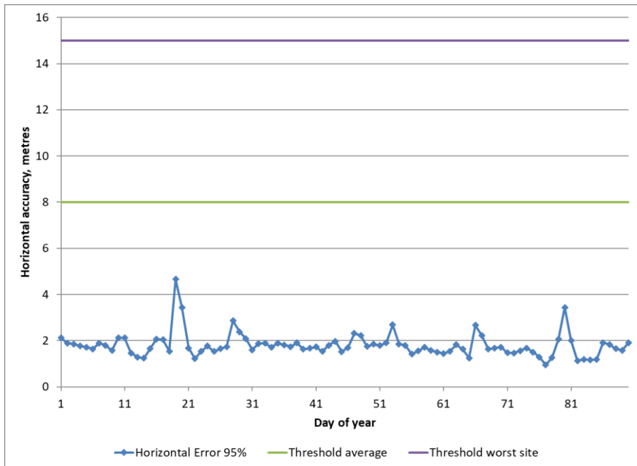
Figure 3-7: Daily Horizontal Position Accuracy (95%) for Reporting Period L1 only
