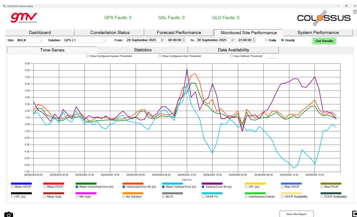
Figure B-1: Hourly Horizontal and Vertical Error Statistics for GPS L1 during 28 to 30 September 2025
