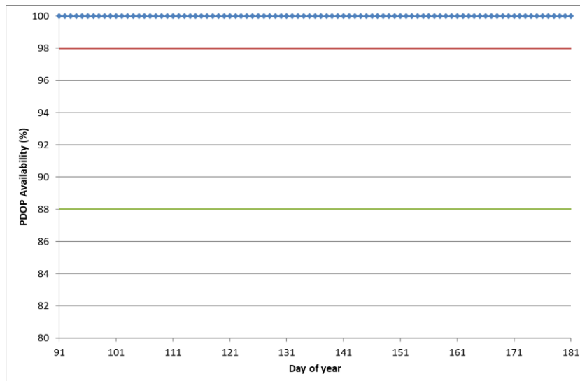
Figure 3-3: Daily PDOP Availability in the Reporting Period
