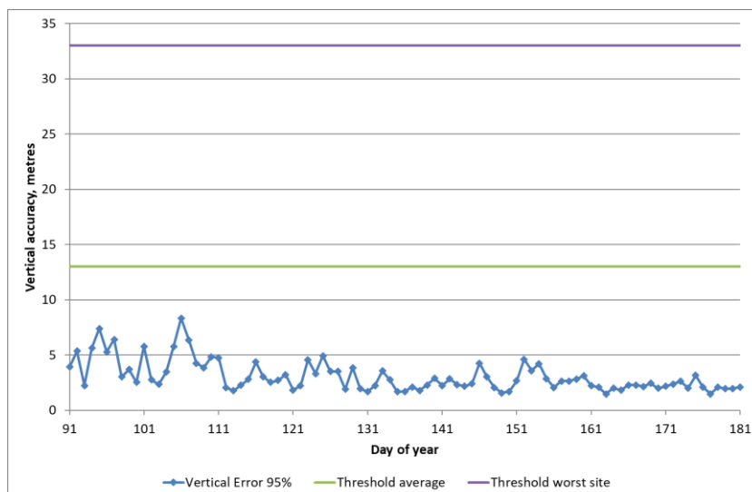
Figure 3-8: Daily Vertical Position Accuracy (95%) for Reporting Period L1 only
