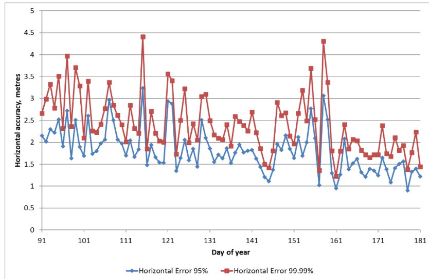
Figure 3-9: Daily Horizontal Position Accuracy (99.99%) for Reporting Period L1 only
