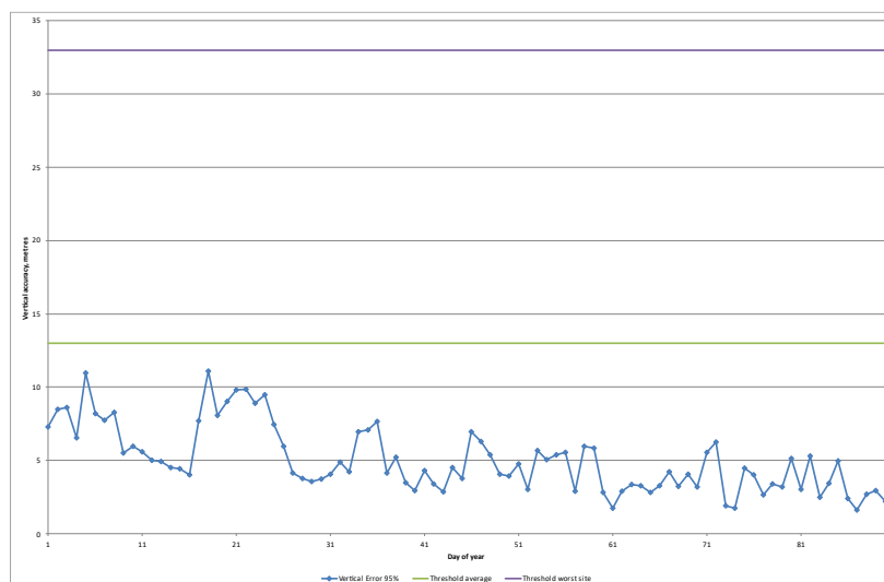
Figure 3-9: Daily Vertical Position Accuracy (95%) for Reporting Period L1 only
