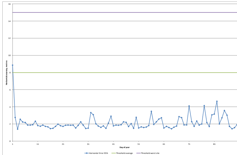
Figure 3-8: Daily Horizontal Position Accuracy (95%) for Reporting Period L1 only
