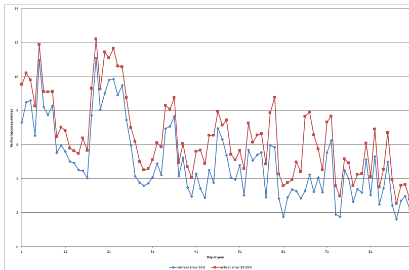
Figure 3-11: Daily Vertical Position Accuracy (99.99%) for Reporting Period L1 only
