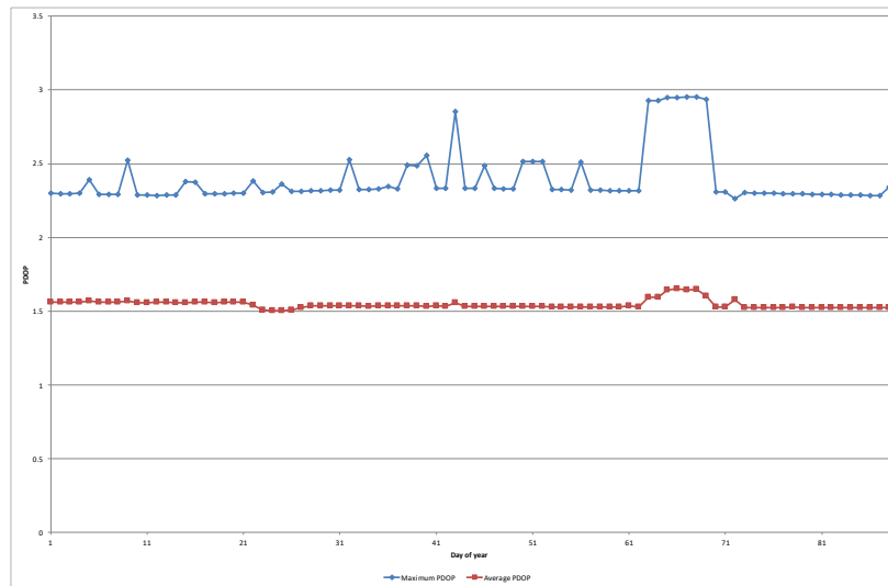
Figure 3-5: Daily Maximum PDOP Value in the Reporting Period
