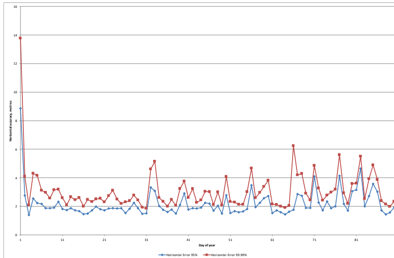
Figure 3-10: Daily Horizontal Position Accuracy (99.99%) for Reporting Period L1 only
