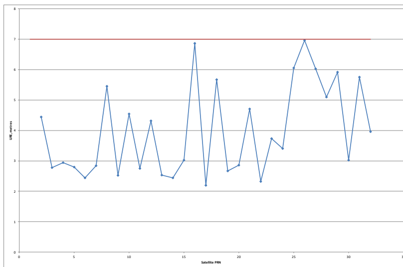
Figure 3-1: Constellation URE (95%) for Reporting Period using L1 only
