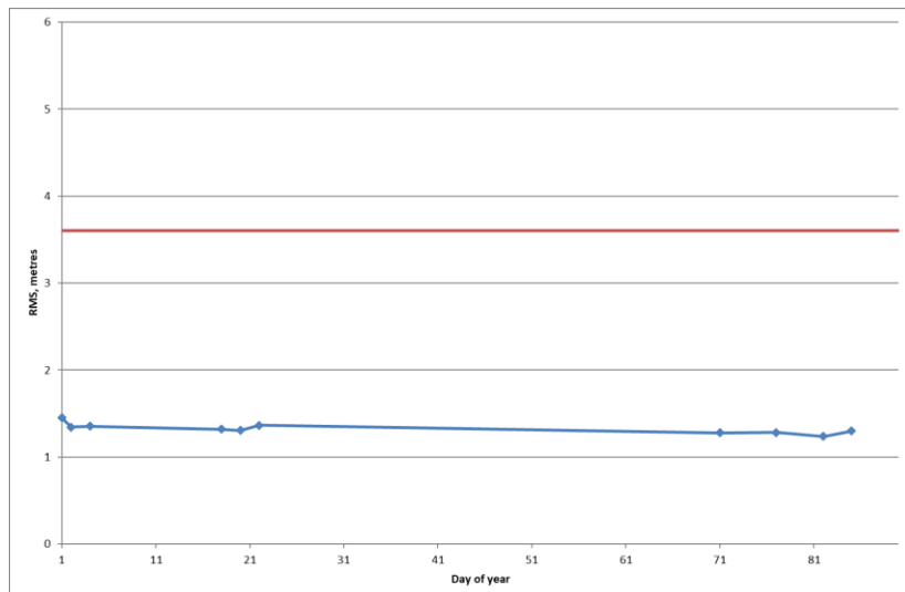
Figure 3-3: Constellation RMS URE for Reporting Period using iono-free combination
