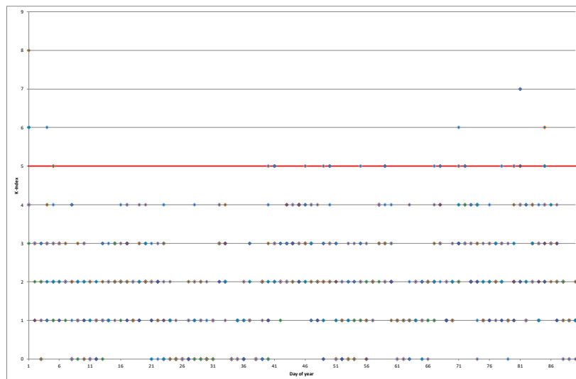
Figure 5-1: K-Index Values at Lerwick during Reporting Period
