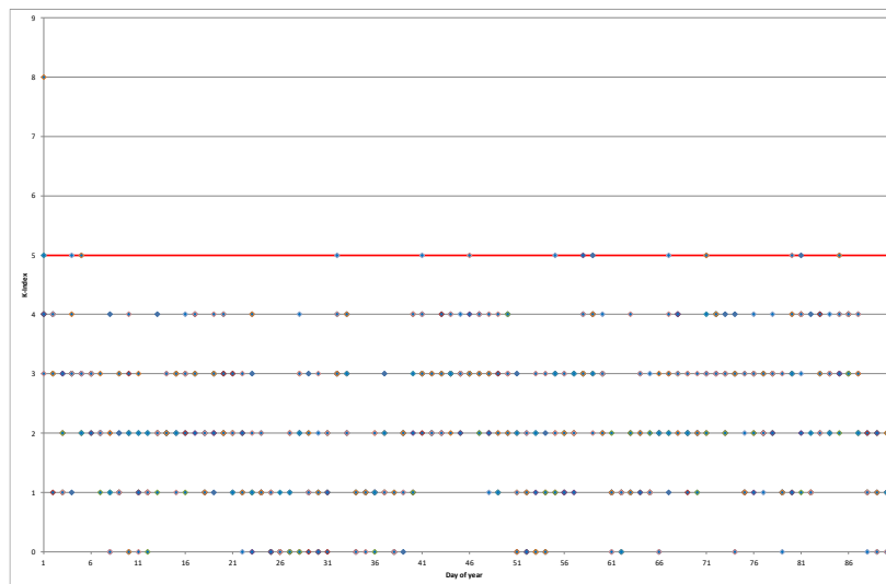
Figure 5-2: K-Index Values at Eskdalemuir during Reporting Period
