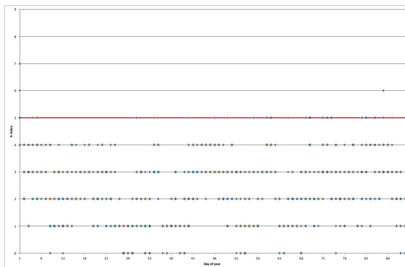
Figure 5-3: K-Index Values at Hartland during Reporting Period
