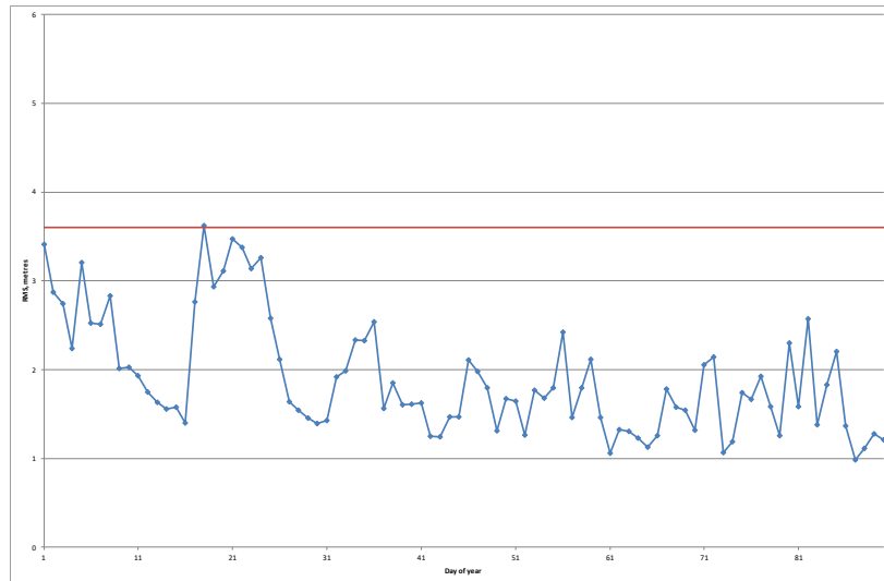
Figure 3-2: Constellation RMS URE for Reporting Period using L1 only
