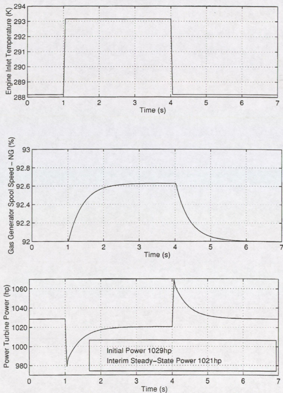
Figure 7(b): Simulated response of a typical helicopter engine to a 5°C change in bulk inlet temperature
