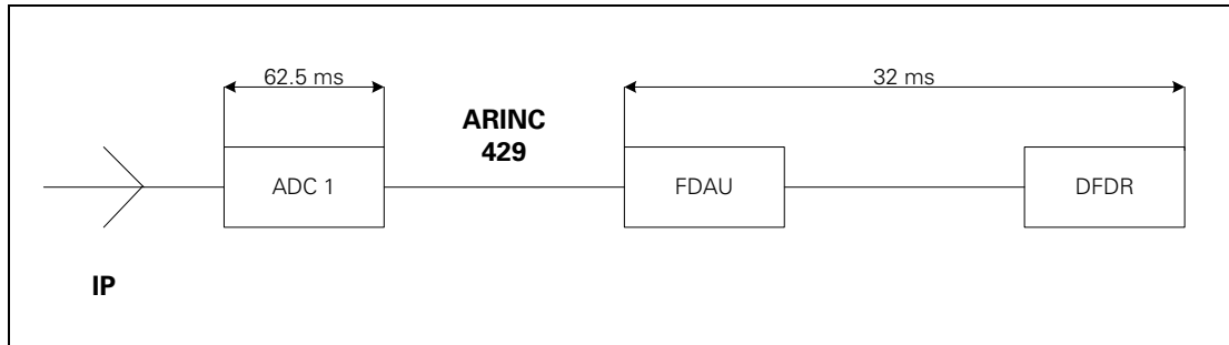
Figure 1 Transport Delay(s)
