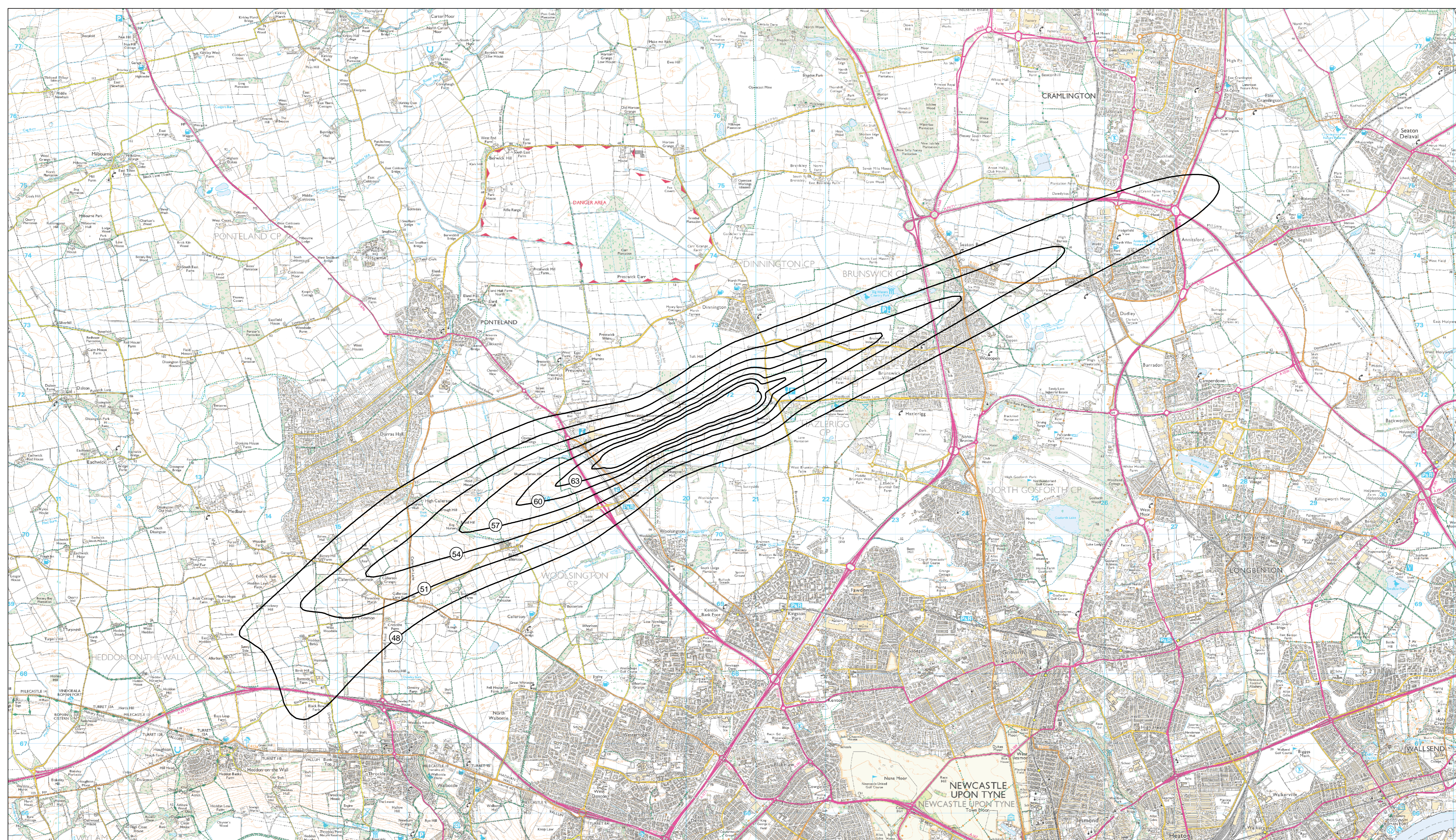
NEWCASTLE INTERNATIONAL AIRPORT Forecast Year 2030 Summer Night L_{Aeq,8hr} Contours Modal Split 75% W / 25% E
