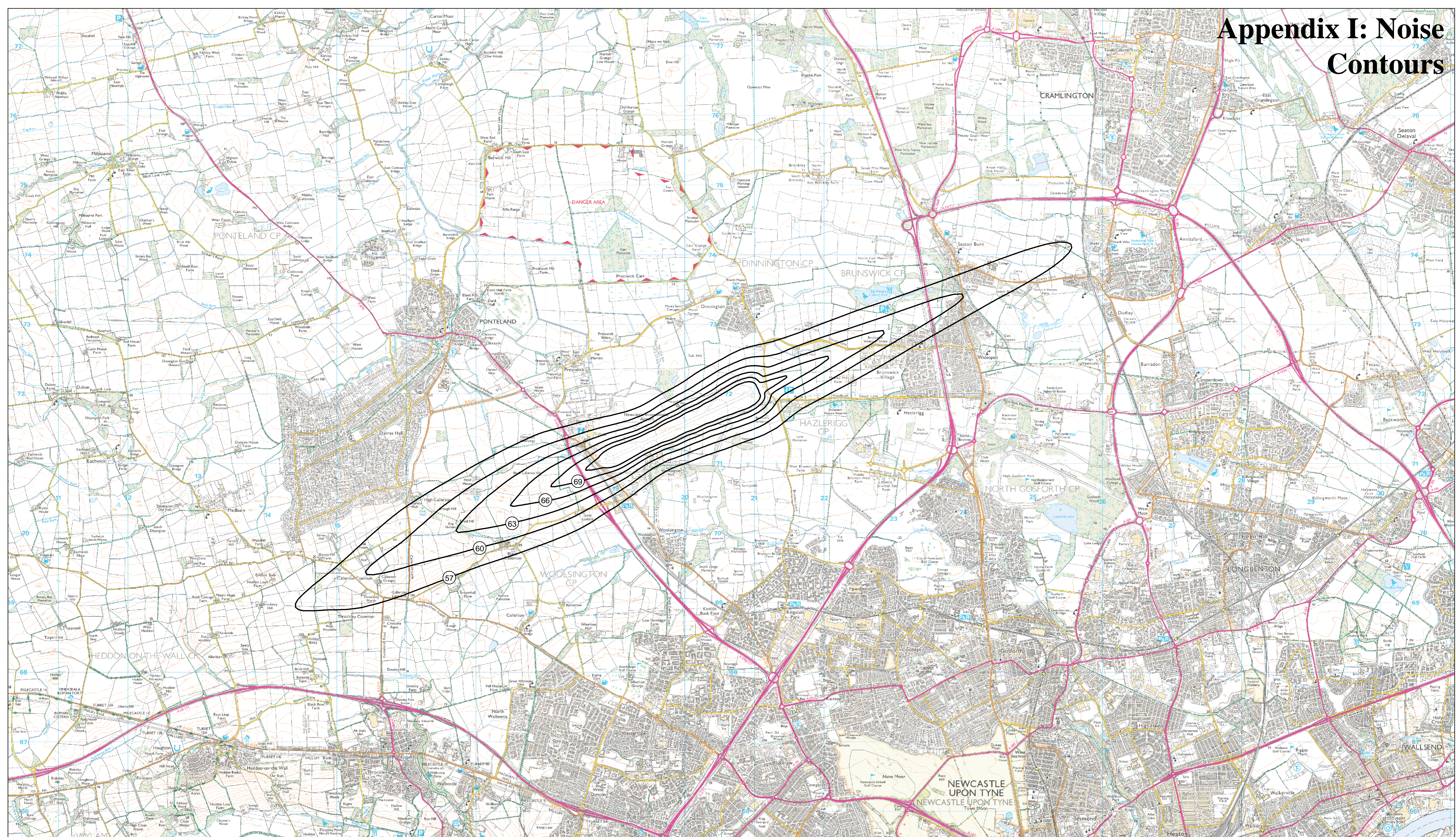
NEWCASTLE INTERNATIONAL AIRPORT Forecast Year 2030 Summer Day L_{Aeq,16hr} Contours Modal Split 75% W / 25% E
